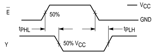
Figure 2. Inverting Switching
