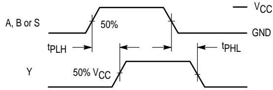
Figure 1. Switching Waveform
