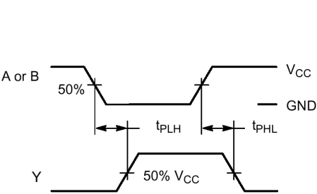
Figure 4. Switching Waveforms
