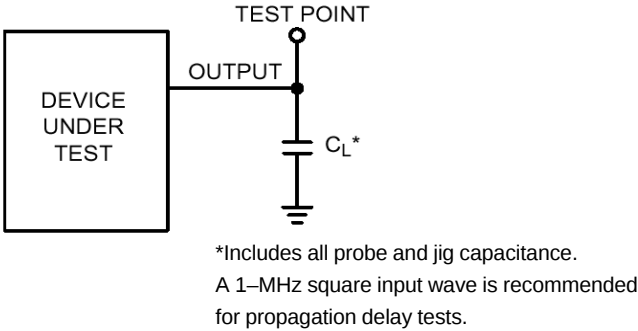
Figure 5. Test Circuit
