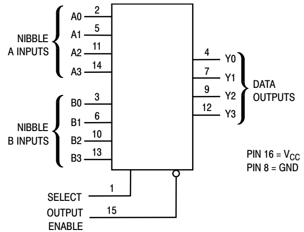
Figure 2. Logic Diagram
