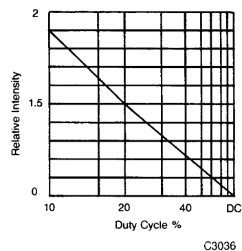
Fig. 6. Luminous Intensity vs. Duty Cycle %
