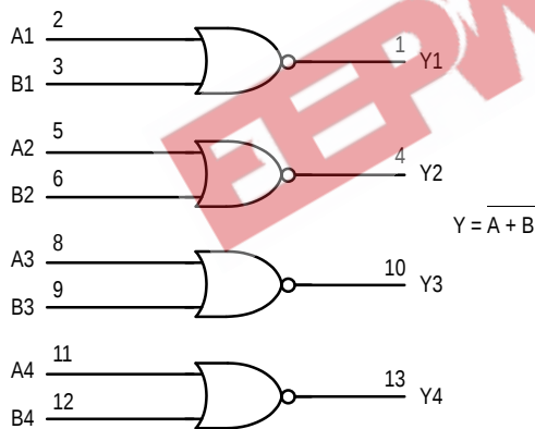
LOGIC DIAGRAM
