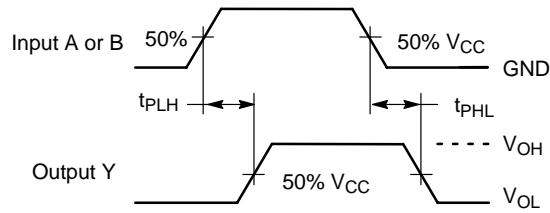
Figure 4. Switching Waveforms
