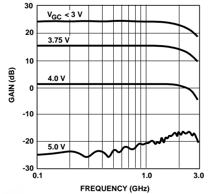
Figure 3. IVA-14228 Gain vs. Frequency and V_{GC} ; V_{CC} = 6V , T_{case} = 25^{\circ}C .
