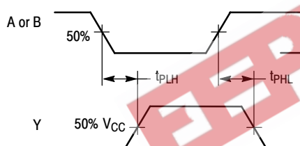
Figure 2. Switching Waveforms
