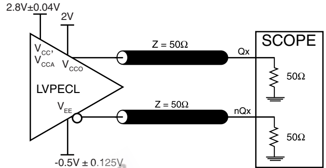
3.3V CORE/2.5V OUTPUT LOAD AC TEST CIRCUIT
