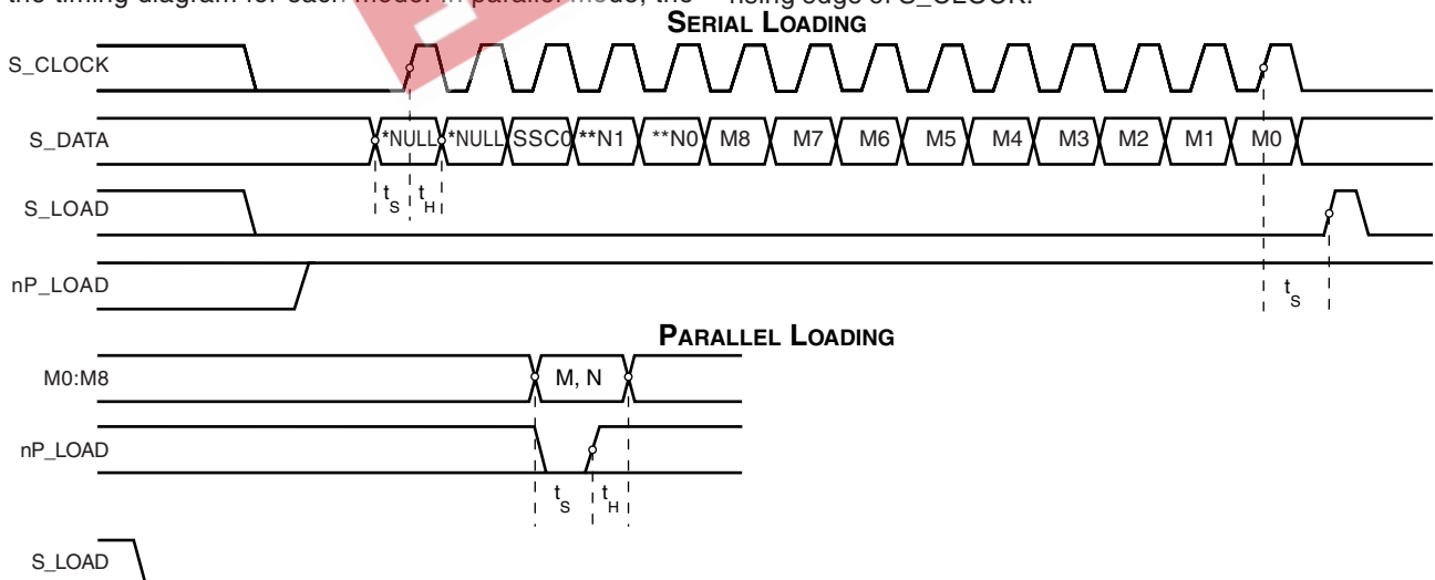
FIGURE 1. PARALLEL & SERIAL LOAD OPERATIONS
