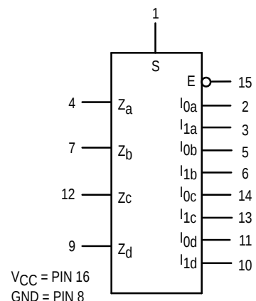
LOGIC SYMBOL
