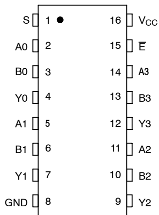
Figure 1. Pin Assignment
