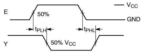
Figure 6. Inverting Switching
