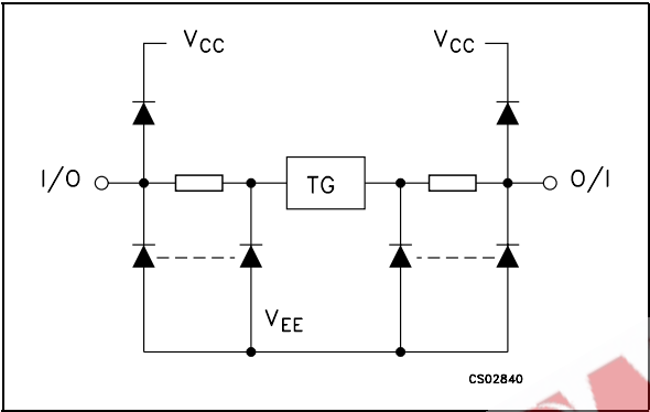
Figure 3: Functional Diagram
