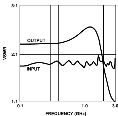
Figure 8. IVA-14228 VSWR vs. Frequency; V CC = 6 V, V GC = 5 V, T case = 25°C.
