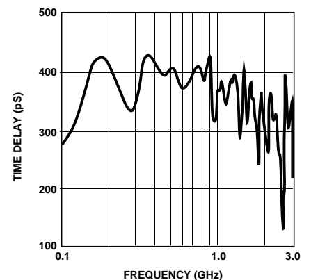
Figure 9. IVA-14228 Group Delay vs. Frequency; V GC = 0 V, V CC = 6 V, T case = 25°C.
