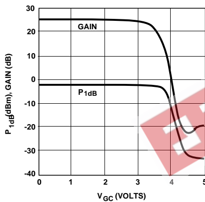
Figure 4. IVA-14228 P 1dB and Gain vs. V GC ; V CC = 6 V, T case = 25°C.
