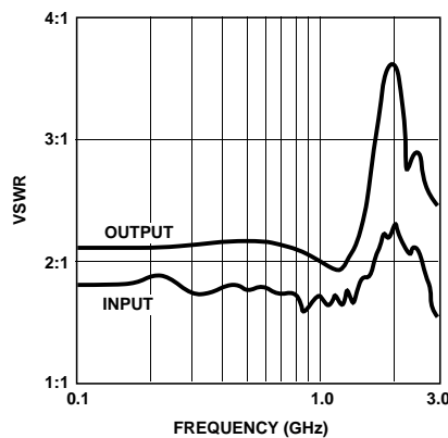
Figure 7. IVA-14228 VSWR vs. Frequency; V CC = 6 V, V GC = 0 V, T case = 25°C.
