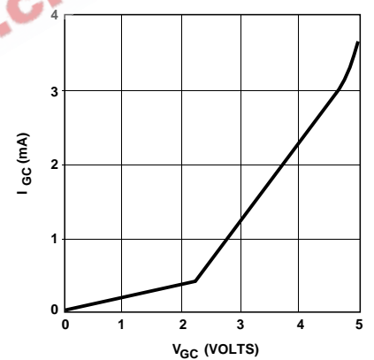
Figure 6. IVA-14228 I GC vs. V GC ; V CC = 6 V, T case = 25°C.
