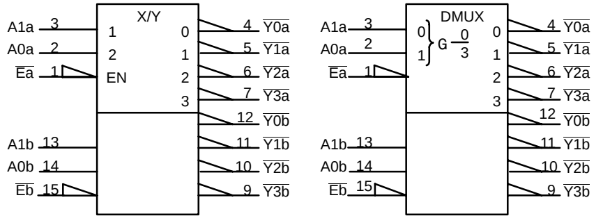
Figure 2. IEC Logic Diagram
