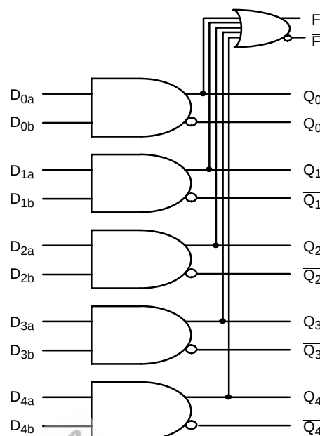
Figure 2. Logic Diagram
