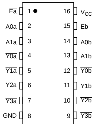
Figure 1. Pin Assignment
