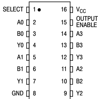
Figure 1. Pin Assignment
