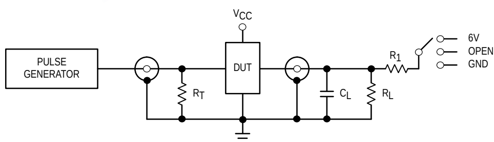
Figure 1. AC Waveforms
