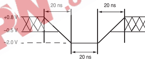
Figure 7.1 Maximum Negative Overshoot Waveform
