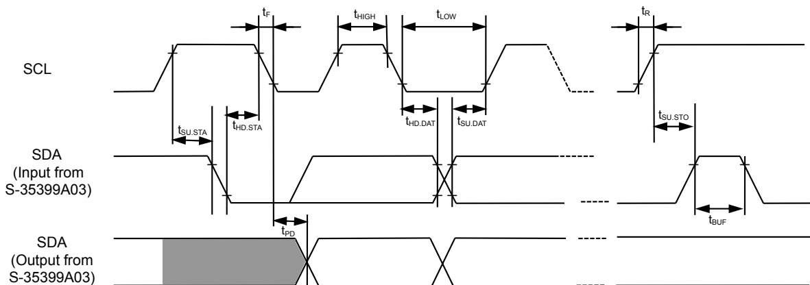
Figure 7 Bus Timing
