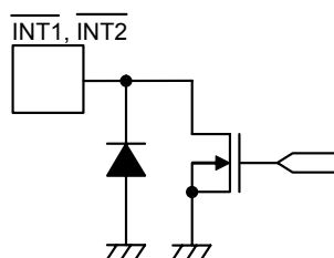
Figure 4 \overline{\text{INT1}} Pin, \overline{\text{INT2}} Pin
