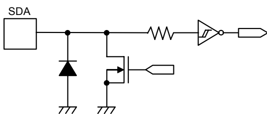
Figure 2 SDA Pin
