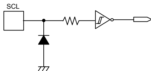
Figure 3 SCL Pin
