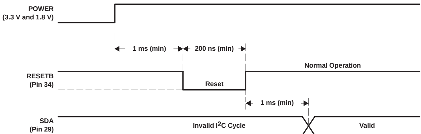
Figure 2–24. Reset Timing
