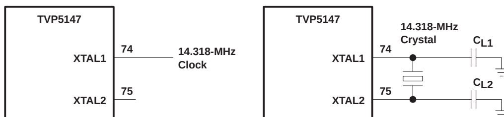
Figure 2-16. Reference Clock Configurations
