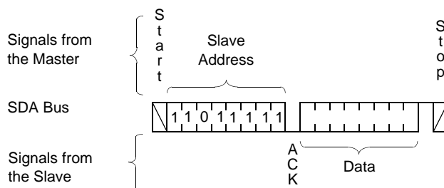
Figure 9. Current Address Read Sequence
