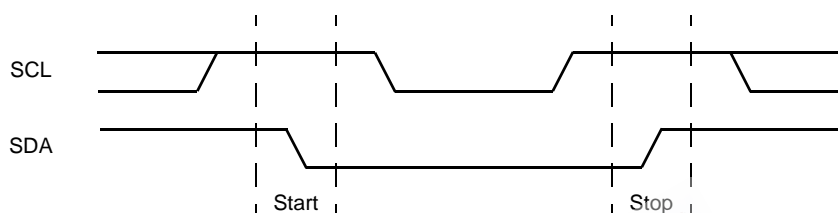
Figure 5. Valid Start and Stop Conditions
