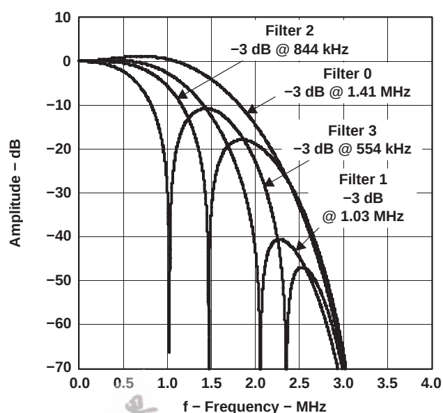
Figure 2-5. Color Low-Pass Filter With Filter Characteristics, NTSC/PAL ITU-R BT.601 Sampling
