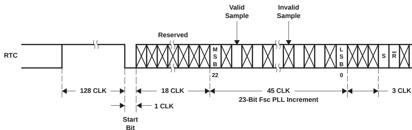
Figure 2–11. RTC Timing
