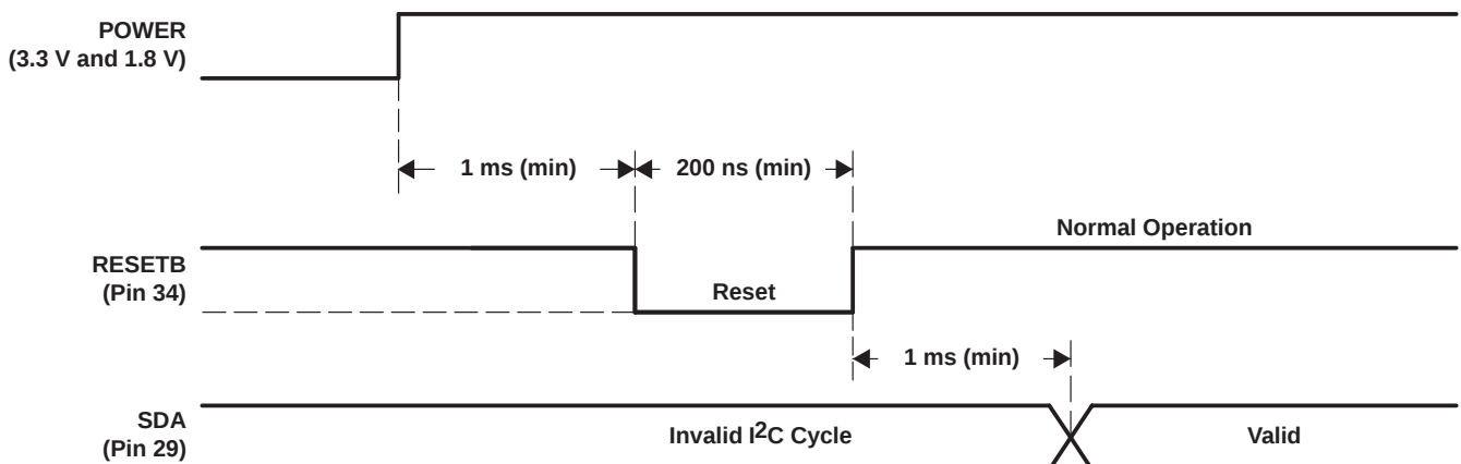
Figure 2–18. Reset Timing
