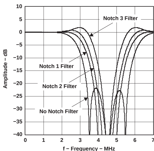
Figure 2-7. Chroma Trap Filter Frequency Response, PAL ITU-R BT.601 Sampling
