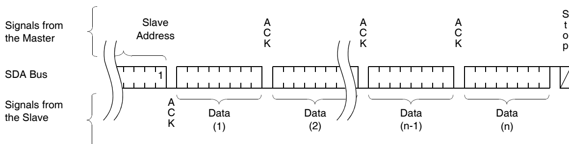
Figure 18. Sequential Read Sequence
