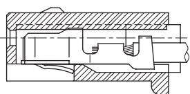
TERMINAL ASSEMBLY DRAWING
