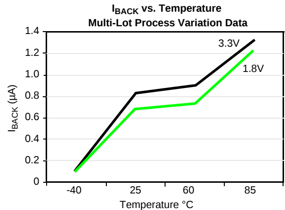
Figure 14. I_{BACK} Performance
