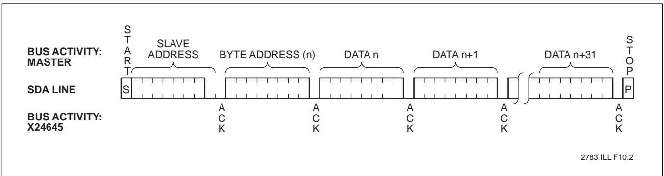
Figure 6. Page Write
