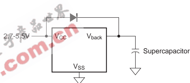
FIGURE 20. SUPERCAPACITOR CHARGING CIRCUIT
