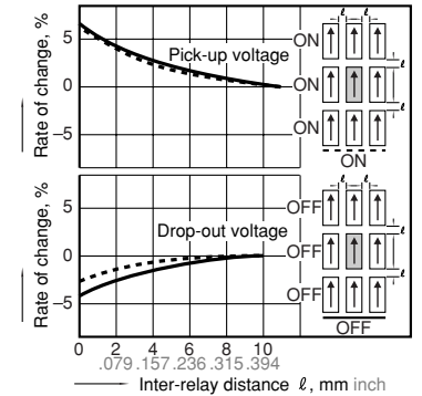
13-(3). Influence of adjacent mounting
