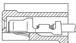
TERMINAL ASSEMBLY DRAWING
