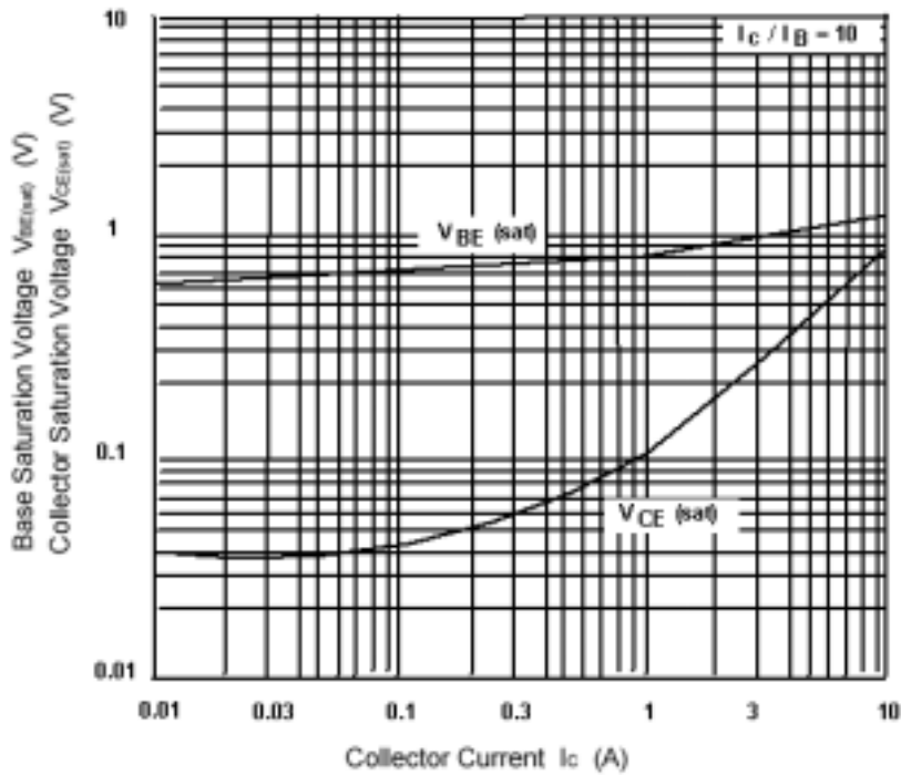
Fig.5 Base-Emitter Saturation Voltage Collector-Emmitter Saturation Voltage
