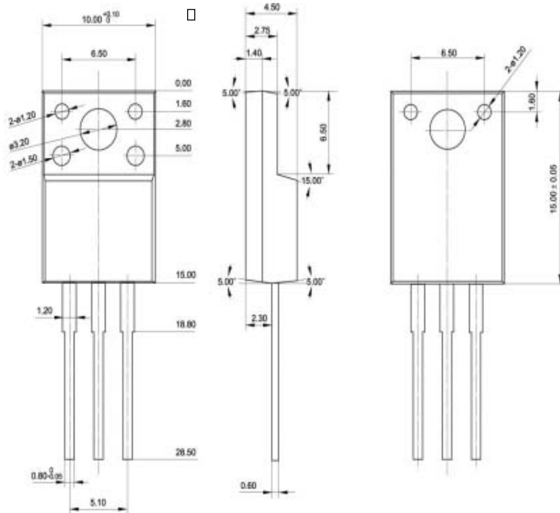
Fig.2 Outline dimensions
