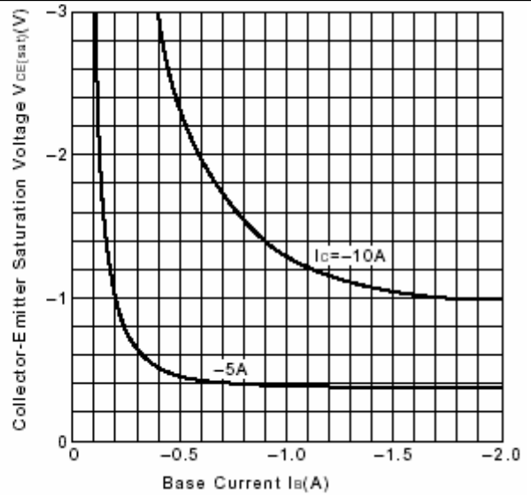
Fig.4 V_{CE(sat)}-I_B Characteristics
