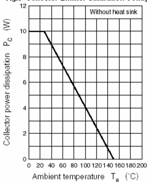
Fig.7 Power Derating
