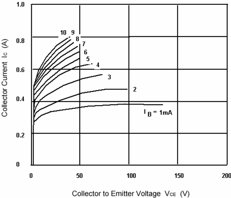
Fig.4 Static Characteristic
