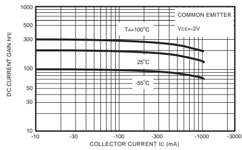
Figure 4. h_{FE} - I_c
