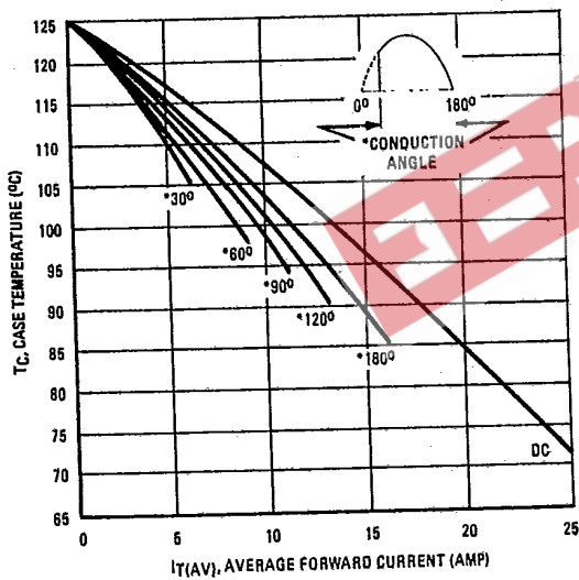
FIGURE 1 - CURRENT DERATING
