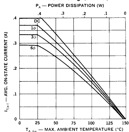
C6 Average Current vs. Ambient Temperature
