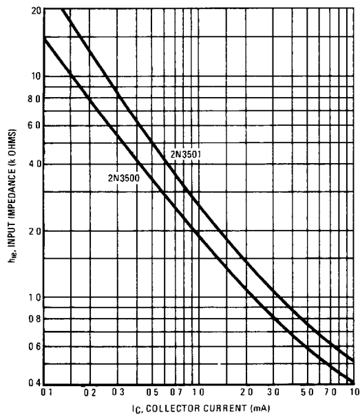
FIGURE 8 — INPUT IMPEDANCE
