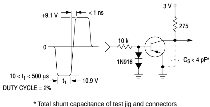
Figure 2. Storage and Fall Time Equivalent Test Circuit
