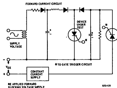
Fig. 17 — Circuit used to measure turn-off time ( t_o ), half-sine-wave pulse.
