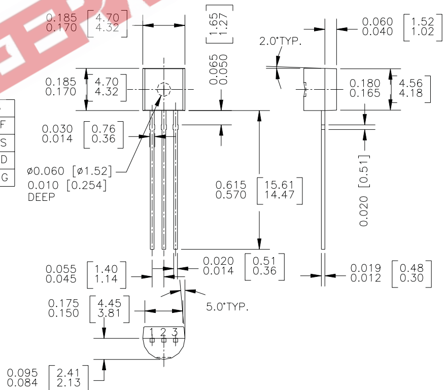
TO-92 (92,94,96)
