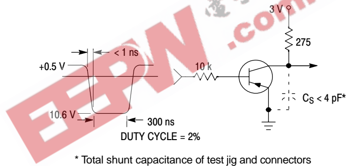
Figure 1. Delay and Rise Time Equivalent Test Circuit
