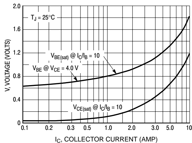
Figure 8. "On" Voltages, MJ2955 (PNP)
