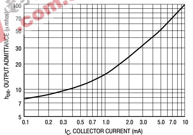
Figure 10. Output Admittance
