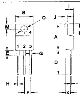
TO-220
