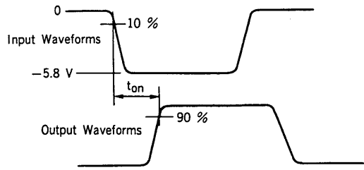
t_{on} Test Waveforms ( V_{BB} = \text{GROUND} )
