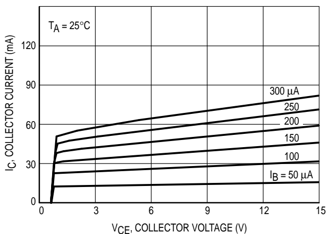
Figure 1. I_C - V_{CE}
