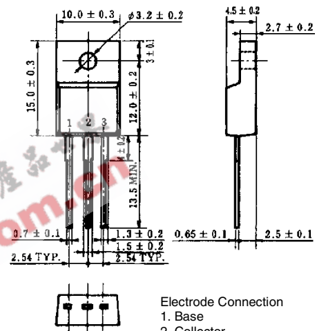
PACKAGE DRAWING (UNIT: mm)
