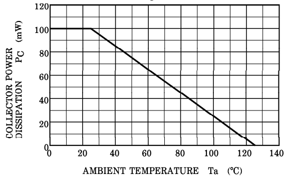
P C - T a
